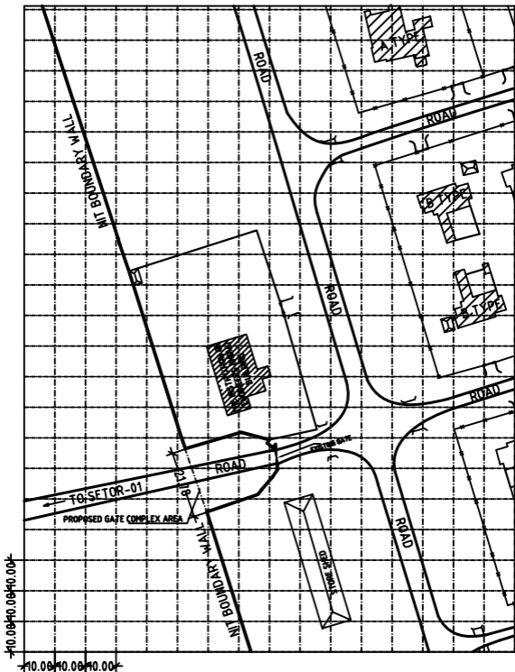
SITE PLAN FOR GATE COMPLEX AT NIT, ROURKELA
